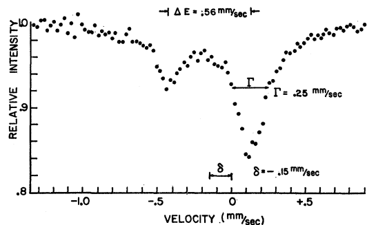
FIG 1. Velocity Spectrum of \text{Co}^{57} in a single-crystal Be sample versus a \text{FeF}_2 absorber (one of the two components of the absorption spectrum) at room temperature. The spectrum was taken parallel to the c axis. The theoretical ratio of the intensities of the components of a two-line quadrupole spectrum parallel to the symmetry axis is 1:3. The observed dips have a smaller intensity ratio, probably due to a slight misalignment of the crystal.
